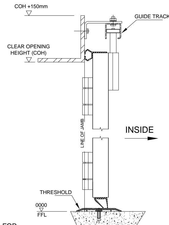
VERTICAL SECTION THROUGH
