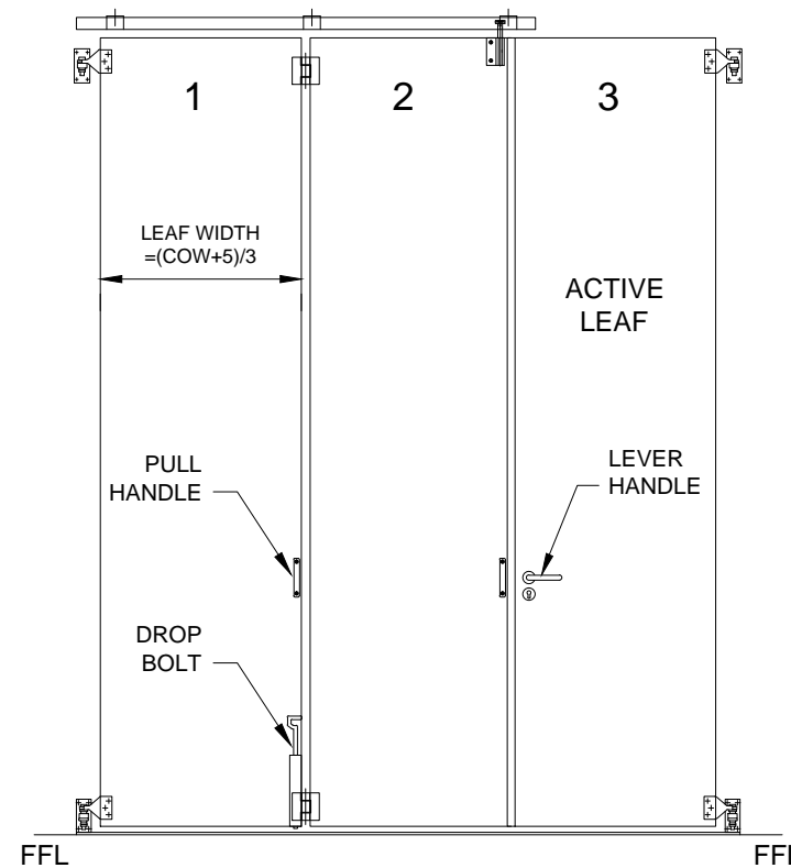
INTERNAL ELEVATION SHOWING STANDARD HARDWARE OPTIONS
