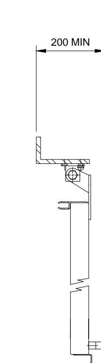
SIDEROOM REQUIRED FOR PULL HANDLE AND DROP BOLT FITTED TO ACTIVE LEAF
