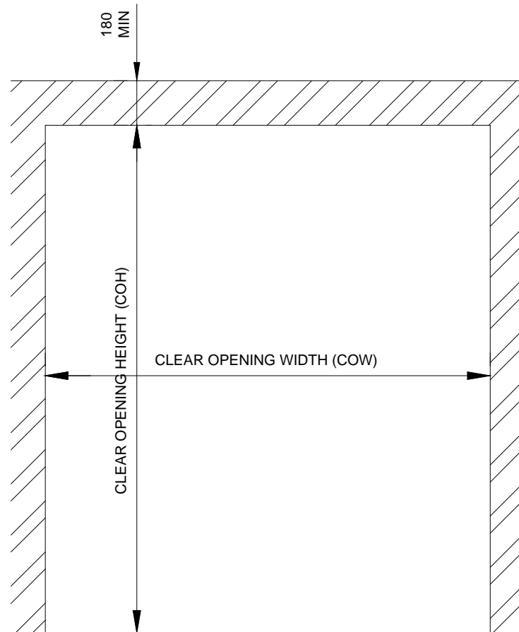
ELEVATION SHOWING INSIDE FACE OF DOOR FRAME
