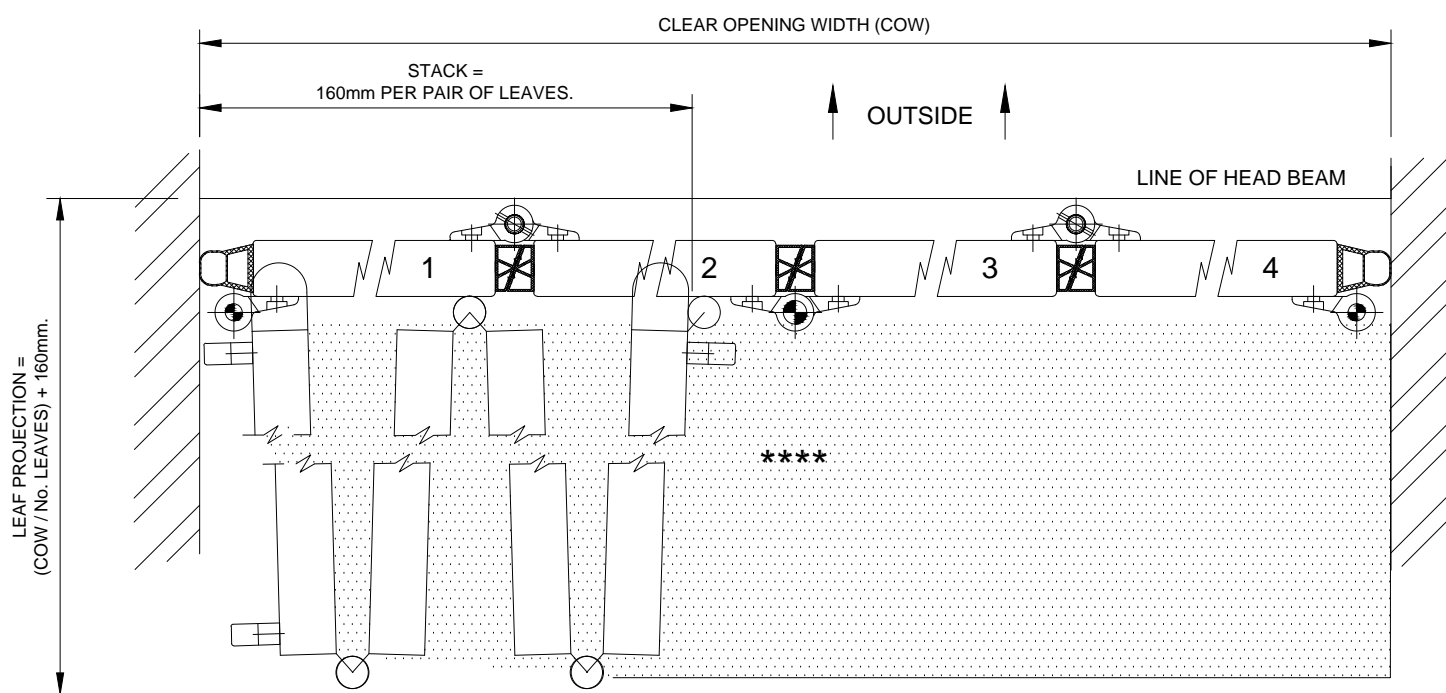
PLAN OF DOOR PANELS IN OPEN AND CLOSED POSITIONS.
