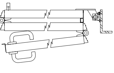
DETAIL SHOWING LEVER FURNITURE FITTED TO ACTIVE LEAF
